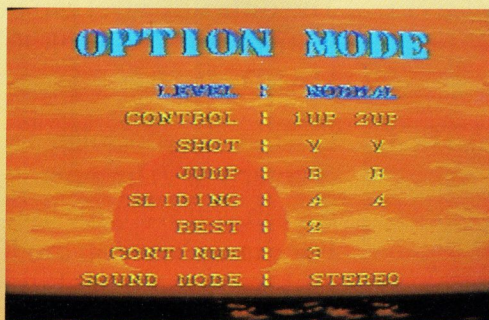
Option Screen
