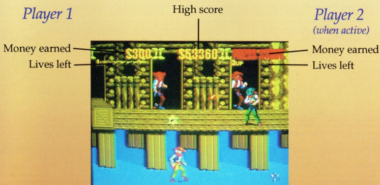
Game Screen
